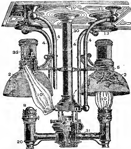
Fig. 3261. Sectional View of Improved Hurricane Chandelier, One Fount, Dual Burners.
